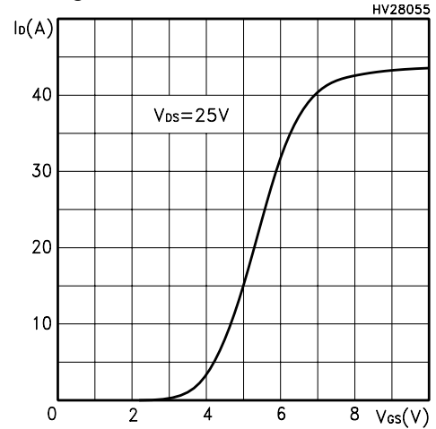
Figure 5: Transfer characteristics
