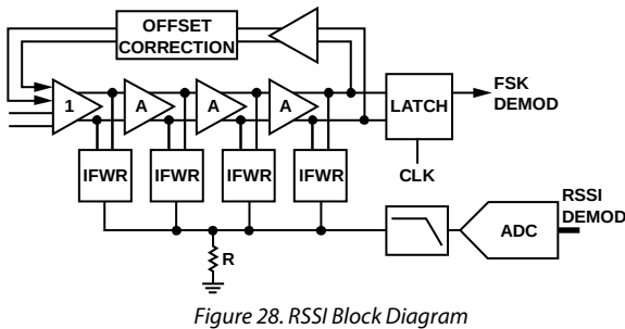
Figure 28. RSSI Block Diagram
