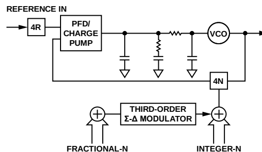
Figure 23. Fractional-N PLL
