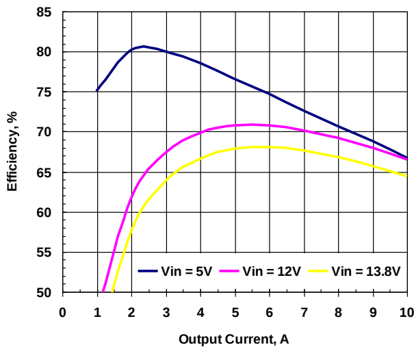
Figure 1. Efficiency vs. Load. V_{out}=0.6V
