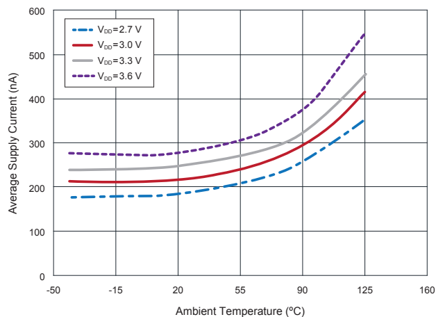
11.2 Average Supply Current vs. Temperature vs. Supply Voltage
