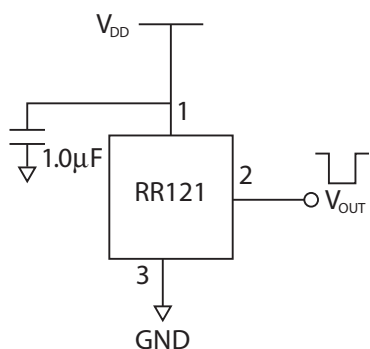
26.1 Application Circuit (SOT-23)
