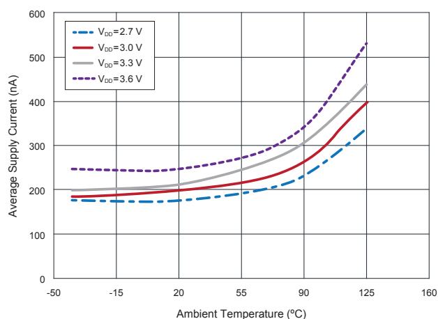
6.2 Average Supply Current vs. Temperature vs. Supply Voltage
