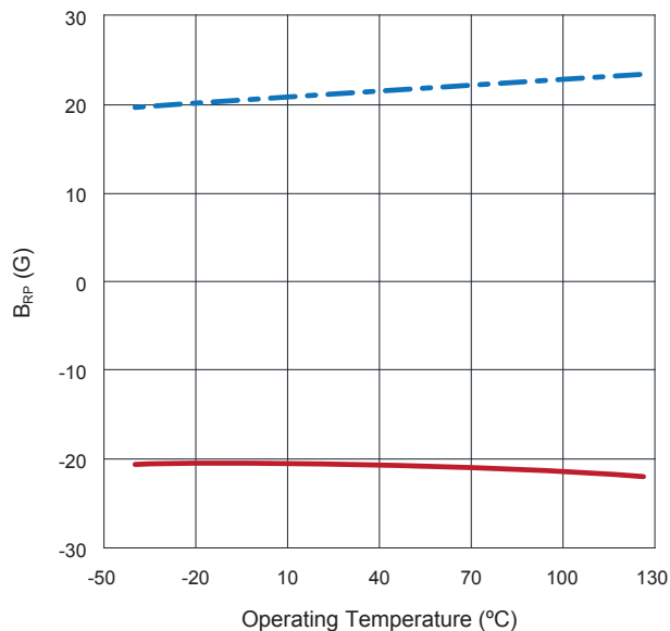
7.4 B_{RPN} (Blue) and B_{RPS} (Red) vs. Operating Temperature at V_{DD}=3.0\text{ V}
