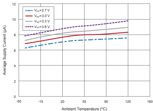
22.2 Average Supply Current vs. Temperature vs. Supply Voltage
