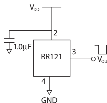
26.2 Application Circuit (LGA-4)
