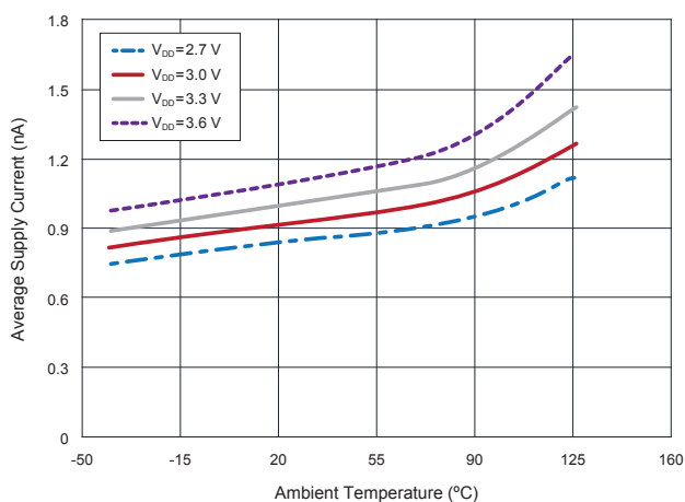
16.2 Average Supply Current vs. Temperature vs. Supply Voltage
