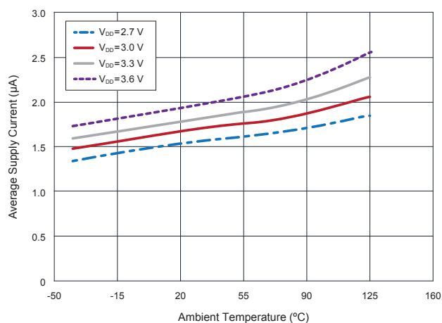
20.2 Average Supply Current vs. Temperature vs. Supply Voltage
