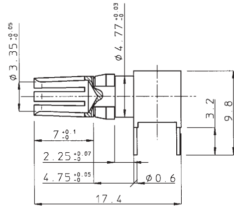
socket contact
