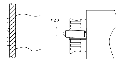
Allowed misalignment
