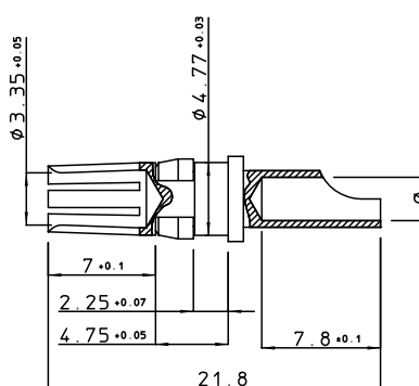
socket contact
