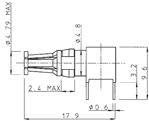
socket contact
