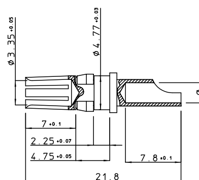
socket contact
