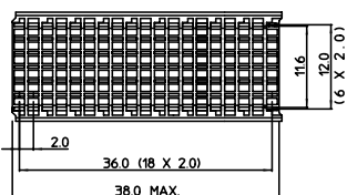
HM2H71P1□□ (type B19)
