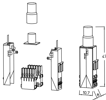
6 x 5 positions
