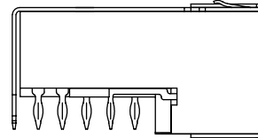
HM2R70PA5108N9 (top shielded only, 4 mm pitch)
