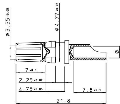
socket contact
