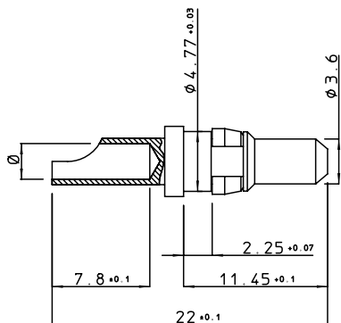
pin contact
