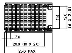
HM2H09P1□□ (type C)
