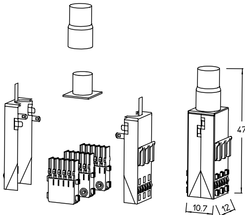
4 x 5 positions
