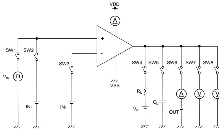
Figure 42. Test Circuit 2
