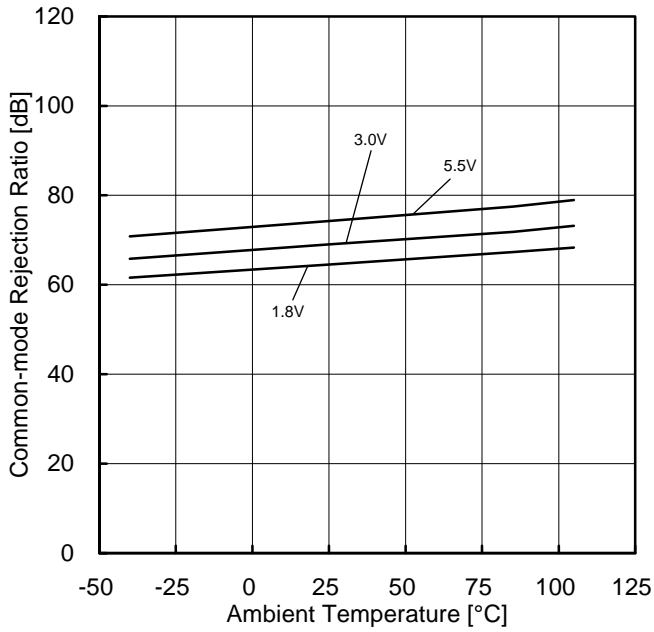
Figure 37. Common-mode Rejection Ratio vs Ambient Temperature
