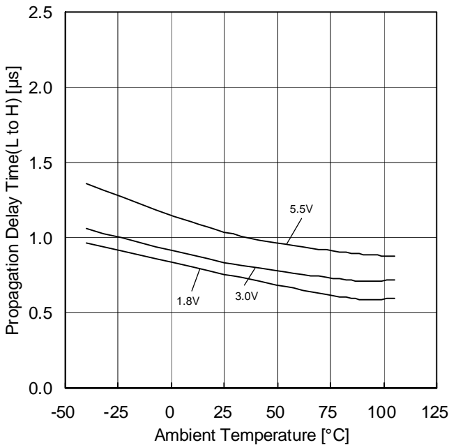
Figure 39. Propagation Delay Time (L to H) vs Ambient Temperature ( R_L=10k\Omega , V_{RL}=3V , C_L=15pF I_N=1.5V , 100mV Overdrive)
