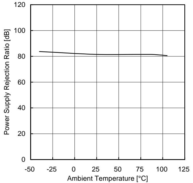
Figure 38. Power Supply Rejection Ratio vs Ambient Temperature
