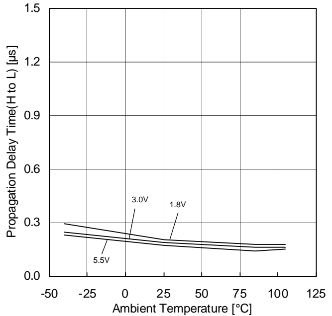
Figure 40. Propagation Delay Time (H to L) vs Ambient Temperature ( R_L=10k\Omega , V_{RL}=3V , C_L=15pF I_N=1.5V , 100mV Overdrive)
