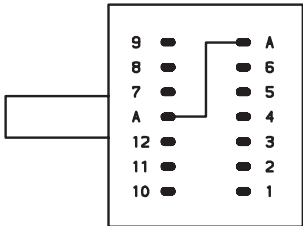
1 POLE 2 - 12 POSITIONS
