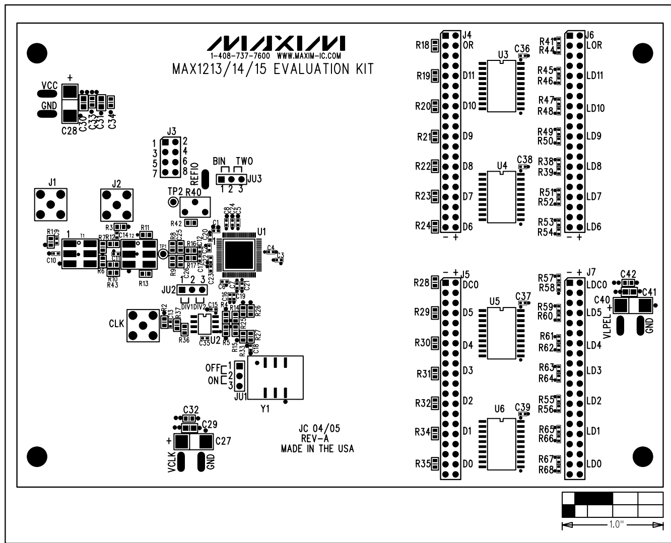
Figure 2. MAX1213/MAX1214/MAX1215 EV Kit Component Placement Guide—Component Side
