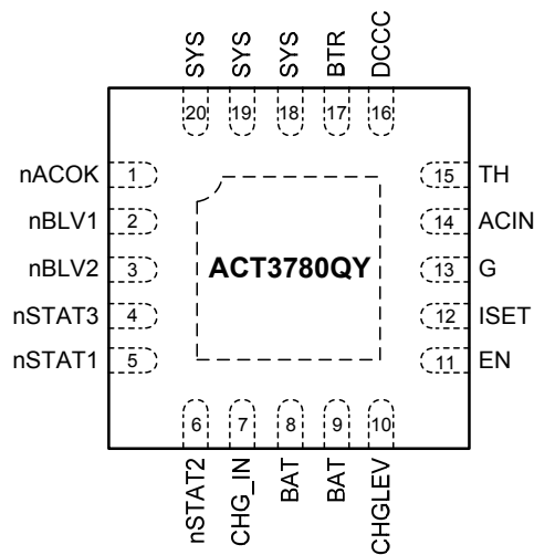
Thin-QFN44-20
