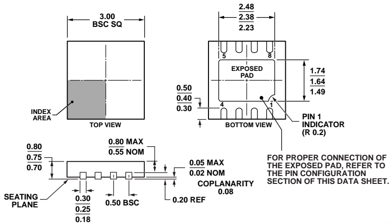
Figure 58. 8-Lead Lead Frame Chip Scale Package [LFCSLP_WD] 3 mm x 3 mm Body, Very Very Thin, Dual Lead (CP-8-5)
