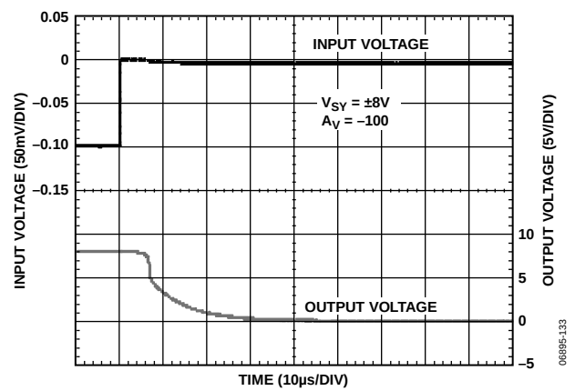
Figure 34. Negative Overload Recovery
