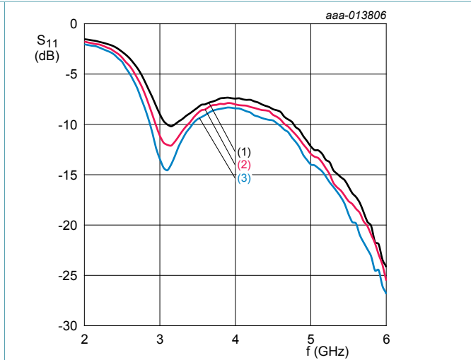
V_{CC} = V_{I(CTRL)} = 3.3 \text{ V} ; gain mode 1. T_{amb} = -40 \text{ }^\circ\text{C} 2. T_{amb} = +25 \text{ }^\circ\text{C} 3. T_{amb} = +85 \text{ }^\circ\text{C}
