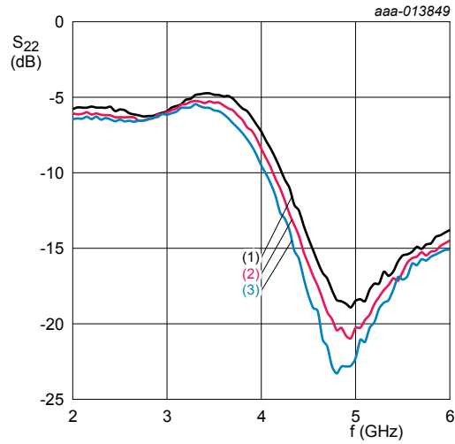
V_{CC} = 3.3\text{ V} ; V_{I(CTRL)} = 0\text{ V} ; bypass mode 1. T_{amb} = -40\text{ °C} 2. T_{amb} = +25\text{ °C} 3. T_{amb} = +85\text{ °C}
