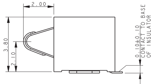
UNDEFLECTED CONTACT
