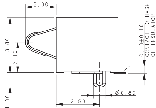
UNDEFLECTED CONTACT
