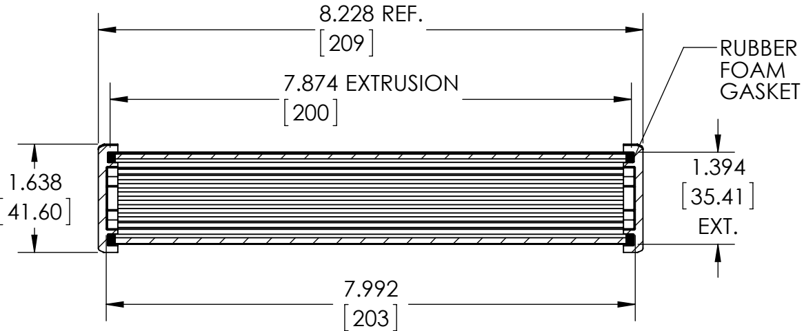
SECTION A-A SCALE 1 : 2 DIMENSIONS MAY VARY DEPENDING ON THE COMPRESSION OF THE GASKETS
