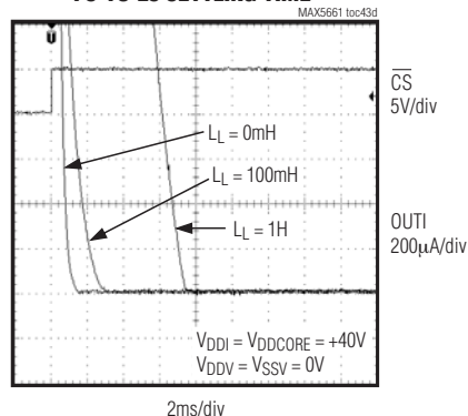
0 TO 20mA CURRENT-OUTPUT, FS-TO-ZS SETTLING TIME
