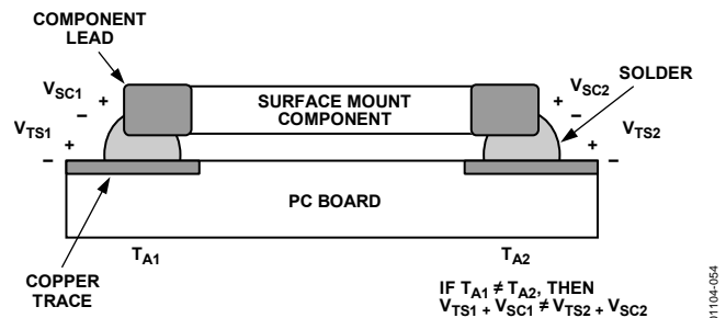
Figure 54. Mismatch in Seebeck Voltages Causes a Thermoelectric Voltage Error
