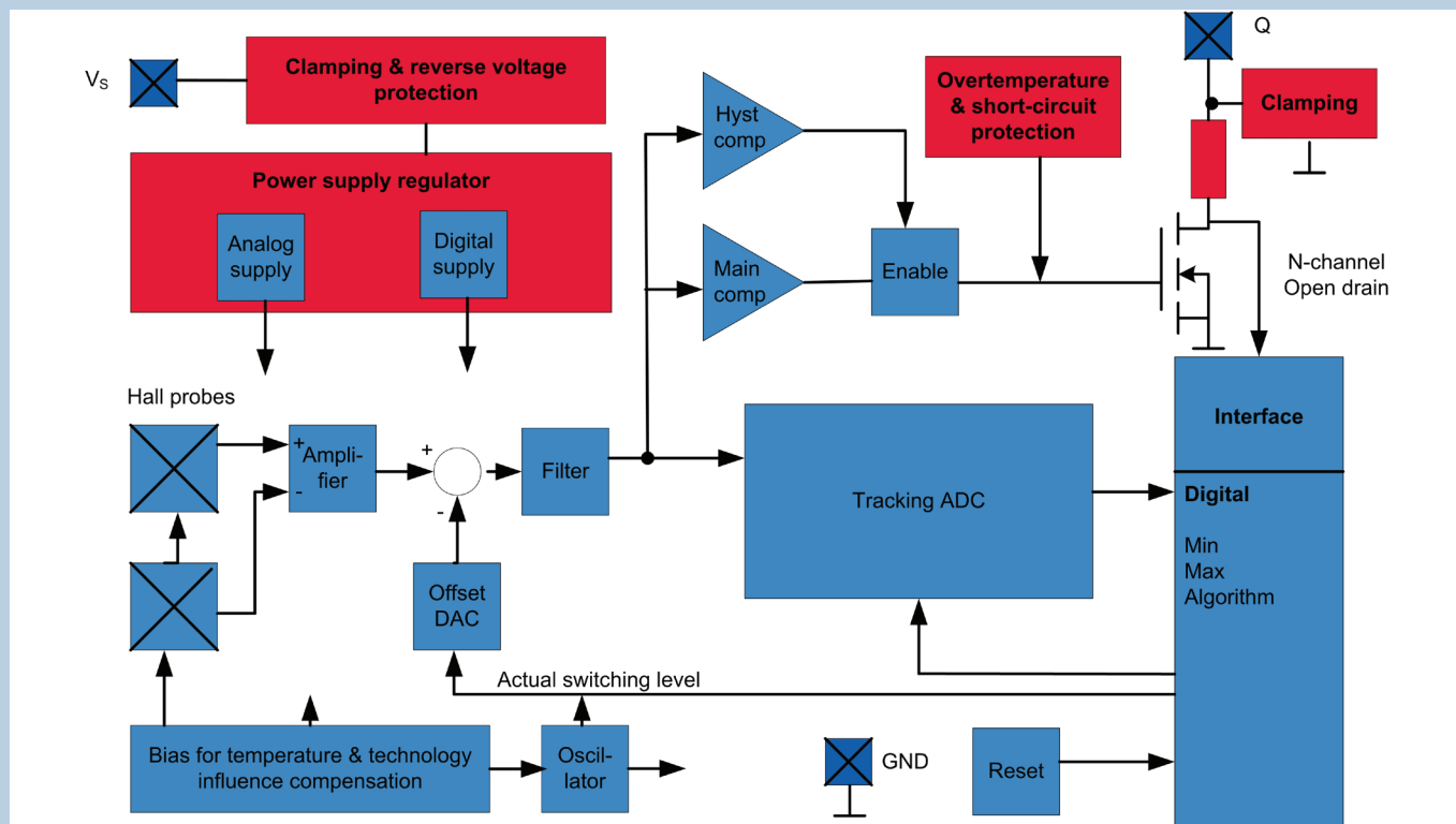
Block Diagram
