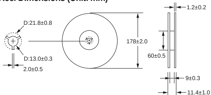
Reel Dimensions (Unit: mm)
