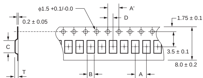
Tape Dimensions (Unit: mm)
