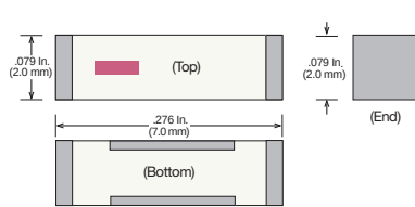
Case 43-2
