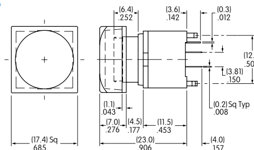
17.4mm Cap
