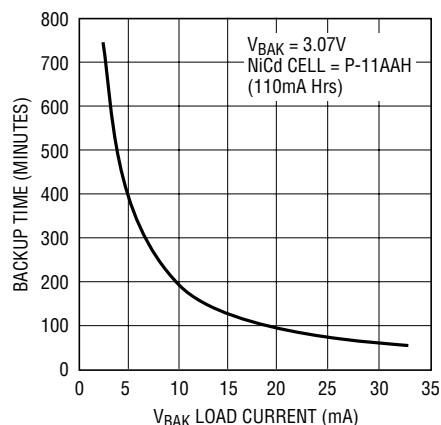
Backup Time vs V BAK Output Load Current
