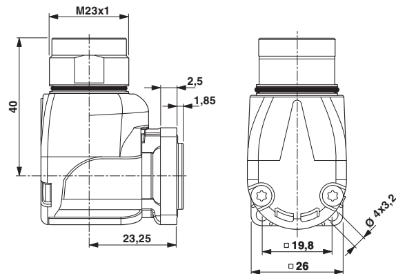
Dimensioned drawing
