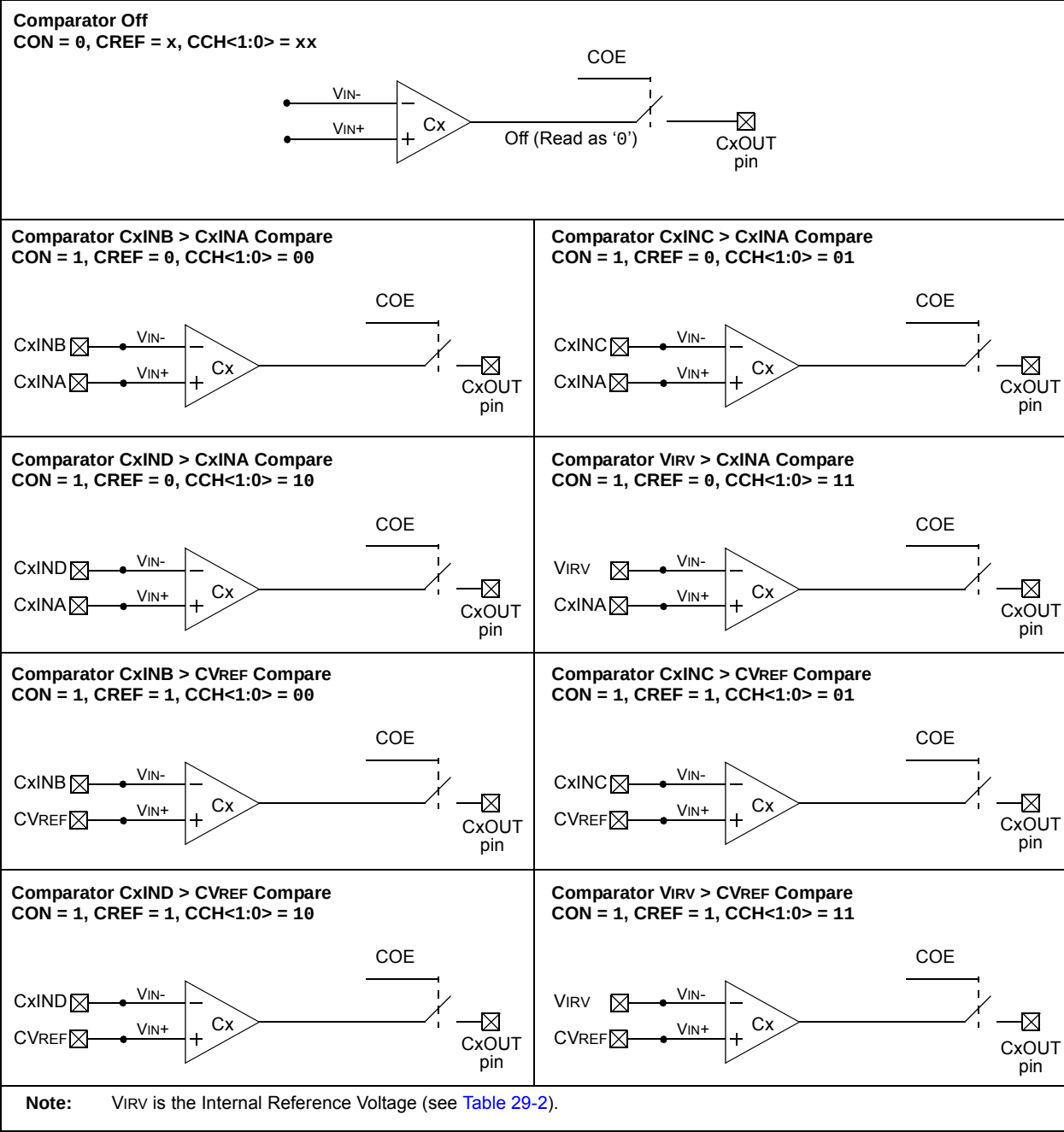
FIGURE 22-4: COMPARATOR CONFIGURATIONS
