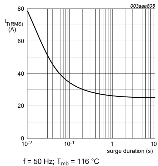
Fig. 2. RMS on-state current as a function of surge duration; maximum values f = 50\text{ Hz} ; T_{mb} = 116\text{ °C}
