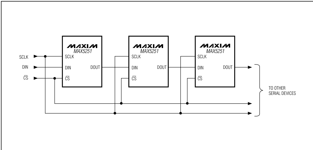
Figure 7. Daisy-Chaining MAX5251s
