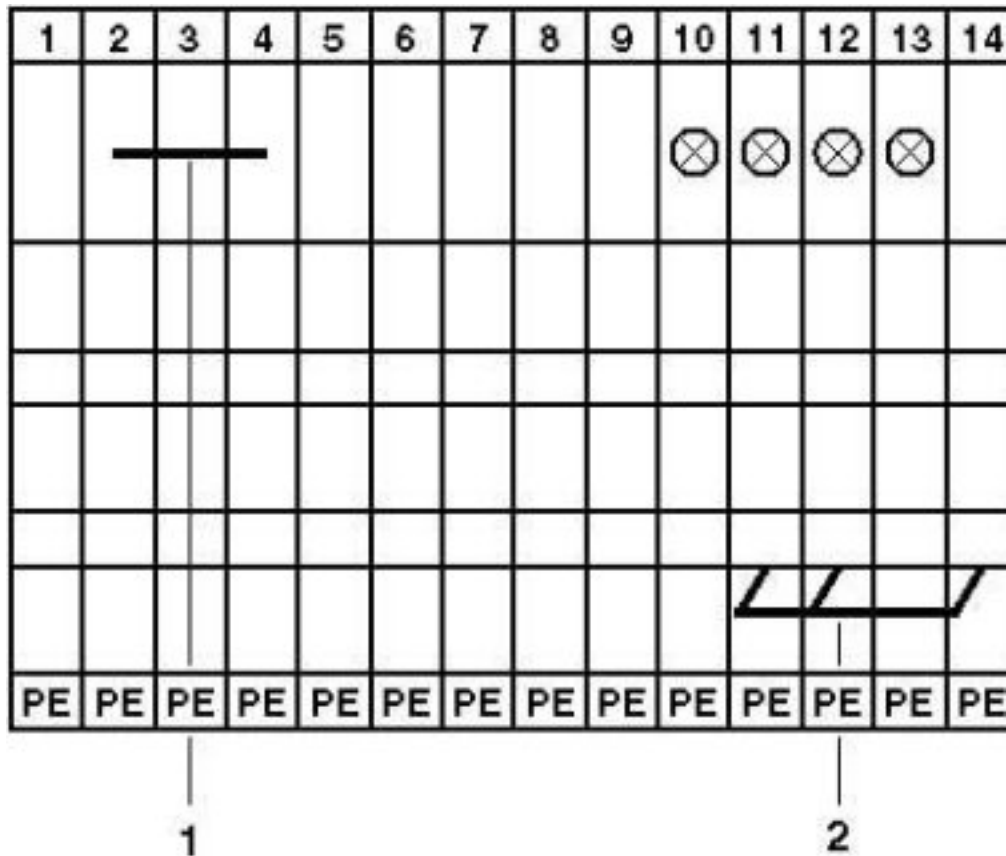
Circuit diagram
