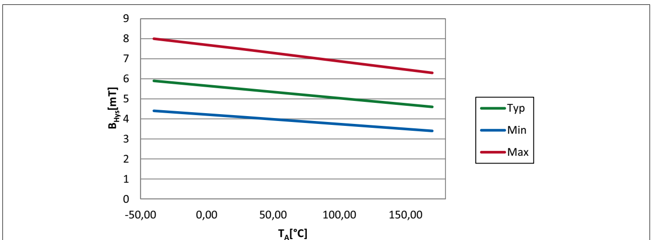
Figure 5-3 Hysteresis ( B_{Hys} ) of the TLE4964-1K over Temperature
