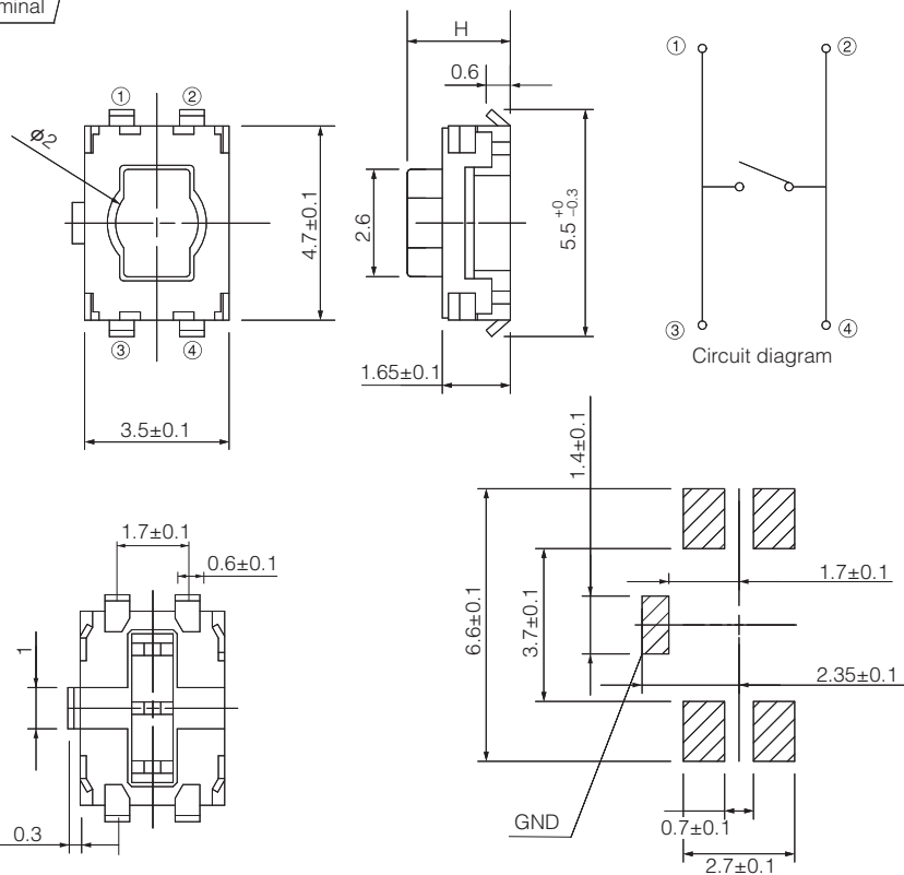
We recommend to connect the GND land shown in the switch spec. with the GND of your P.C.B for withstanding electric-static discharge.
