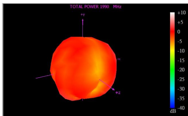
1990 MHz
