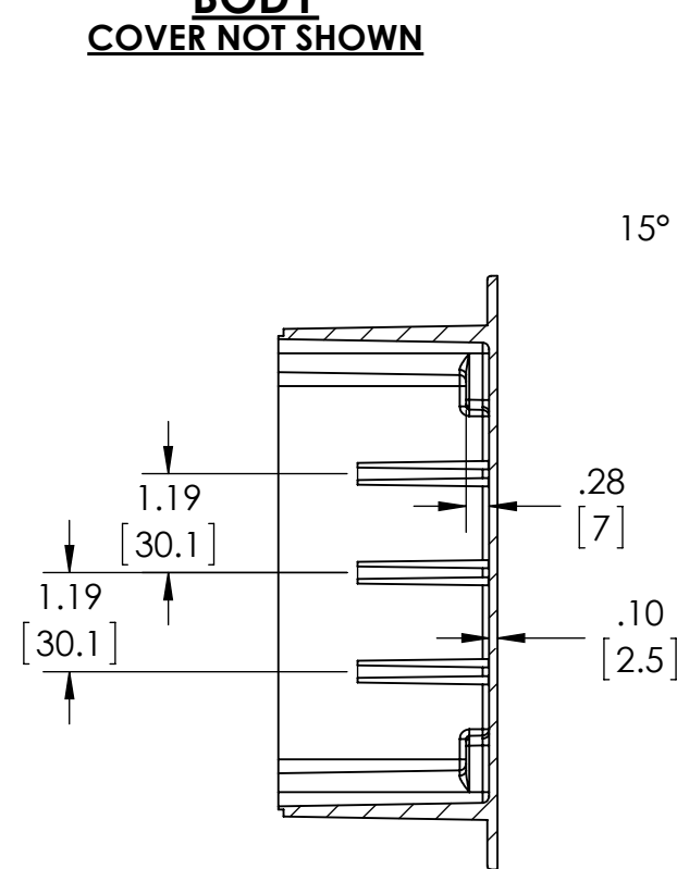
SECTION B-B
