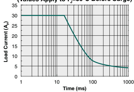
Maximum Surge Current (non-Repetitive) (Values Apply to T_j=50°C Before Surge)
