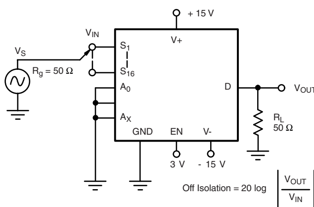
Figure 6. Off Isolation
