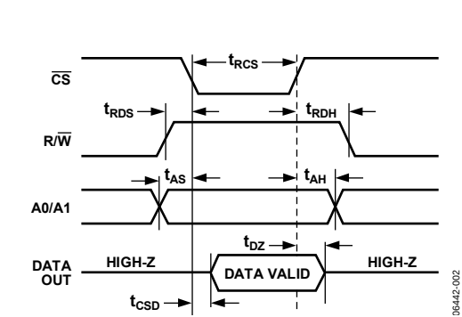
Figure 2. Data Read Timing
