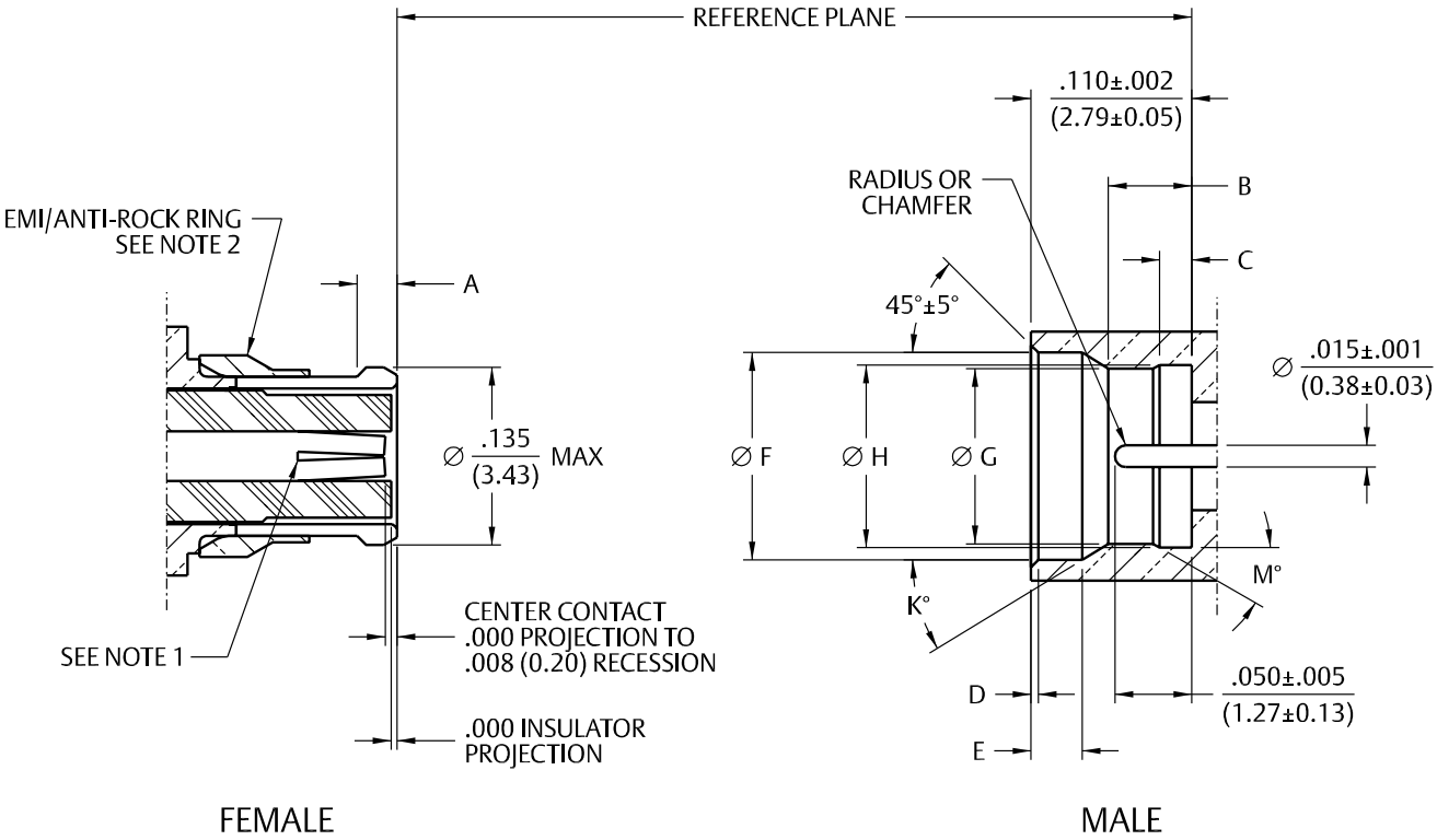
Mating Engagement for SMP Series per MIL-STD-348A
