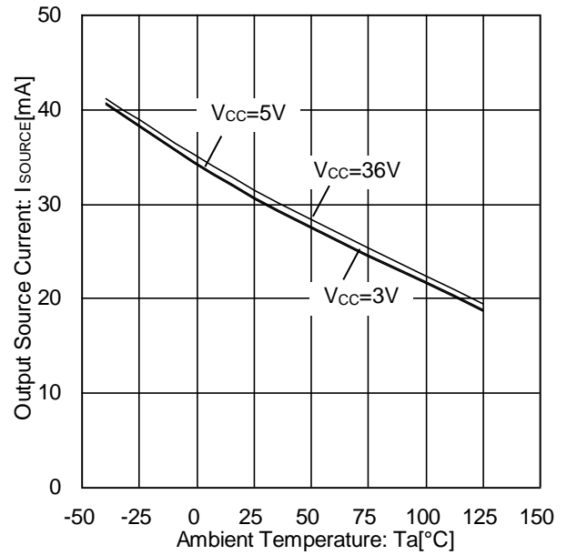
Figure 30. Output Source Current vs Ambient Temperature ( V_{OUT}=0V )
