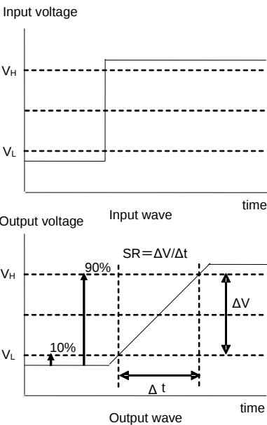
Figure 50. Slew Rate Waveform
