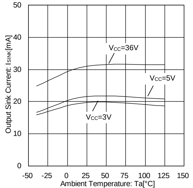
Figure 9. Output Sink Current vs Ambient Temperature ( V_{OUT}=V_{CC} )
