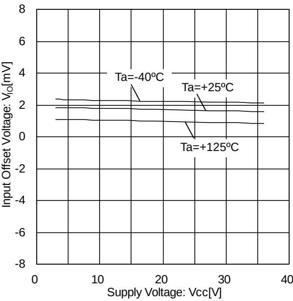
Figure 12. Input Offset Voltage vs Supply Voltage (V ICM =0V, V OUT =1.4V)
