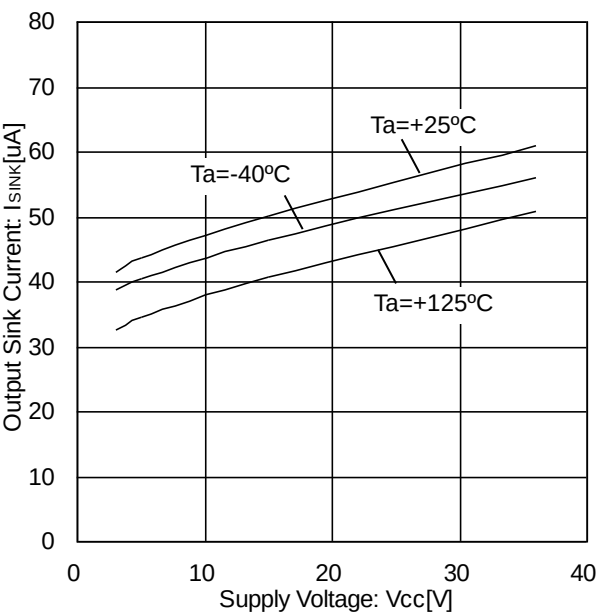
Figure 10. Output Sink Current vs Supply Voltage (V OUT =0.2V)
