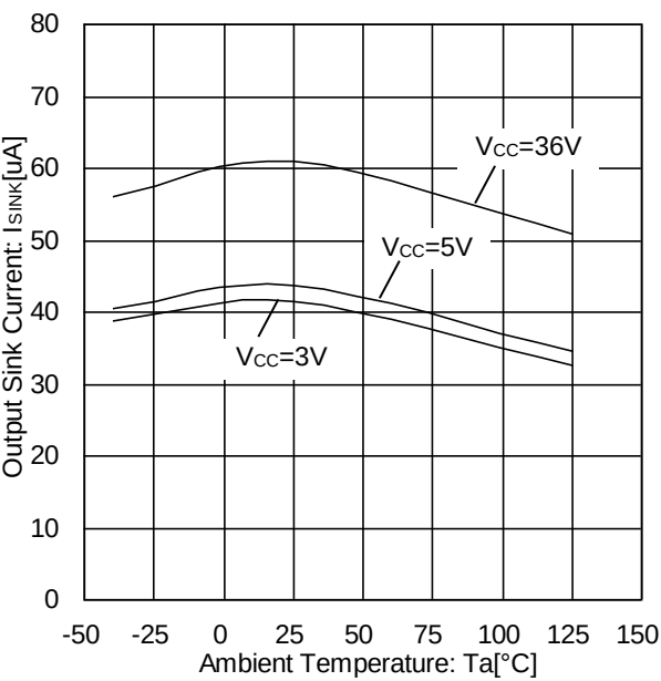
Figure 11. Output Sink Current vs Ambient Temperature (V OUT =0.2V)
