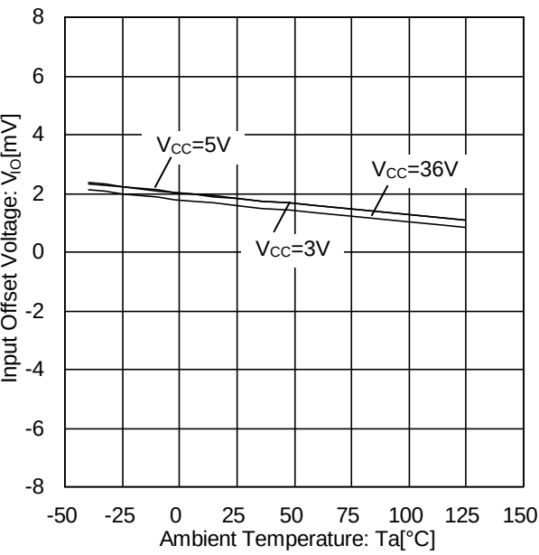
Figure 13. Input Offset Voltage vs Ambient Temperature (V ICM =0V, V OUT =1.4V)
