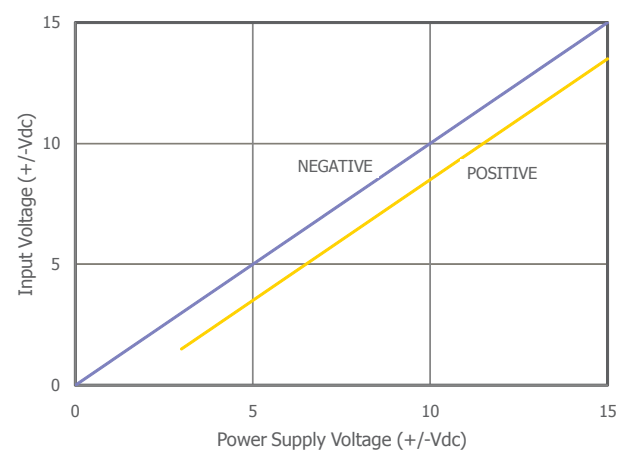
Input Voltage Range vs. Power Supply
