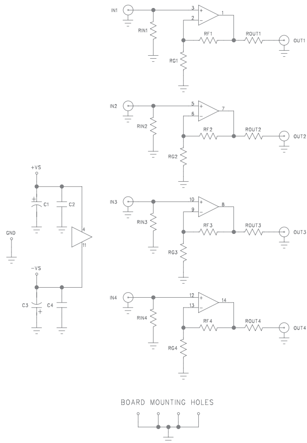
Figure 13. CEB018 Schematic
