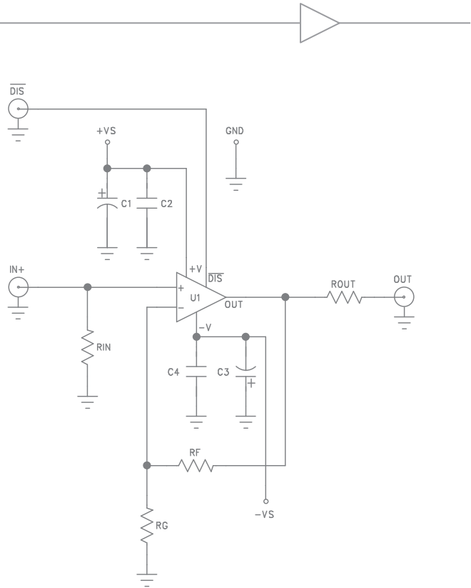
Figure 7. CEB002 Schematic
