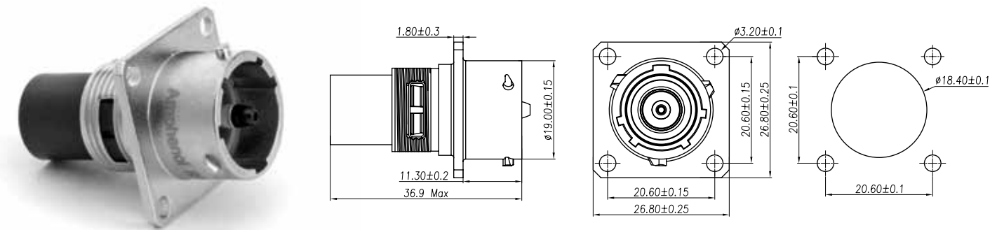
Wall Mounting Receptacle for Crimp Barrel
