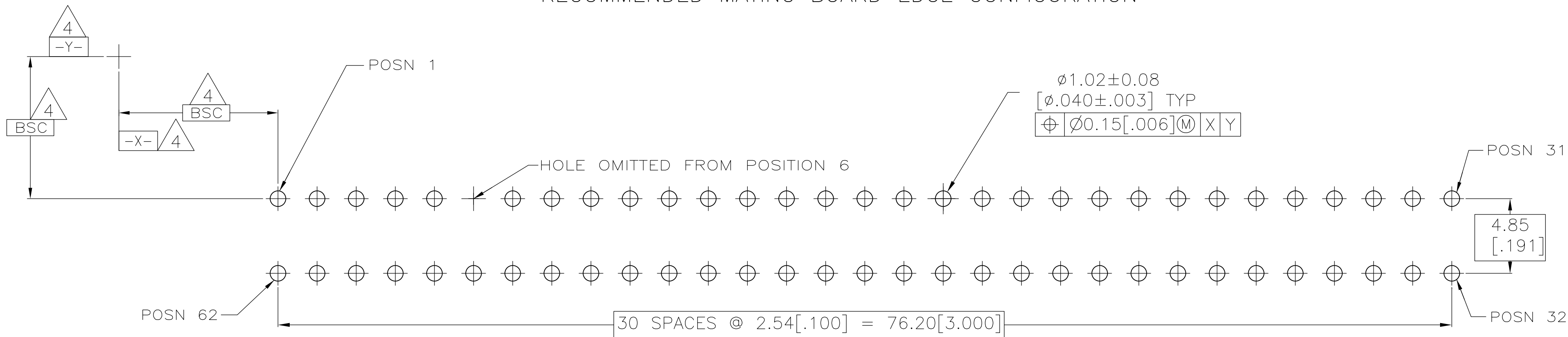
RECOMMENDED MATING BOARD EDGE CONFIGURATION
