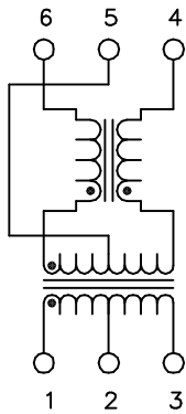
SCHEMATIC
