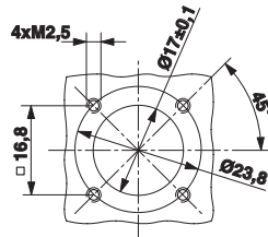
Dimensioned drawing
