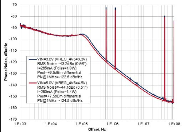
Figure 10. Phase noise and fractional spurs at 11502.5 MHz vs. supply ( F_{PFDD}=50 MHz)
