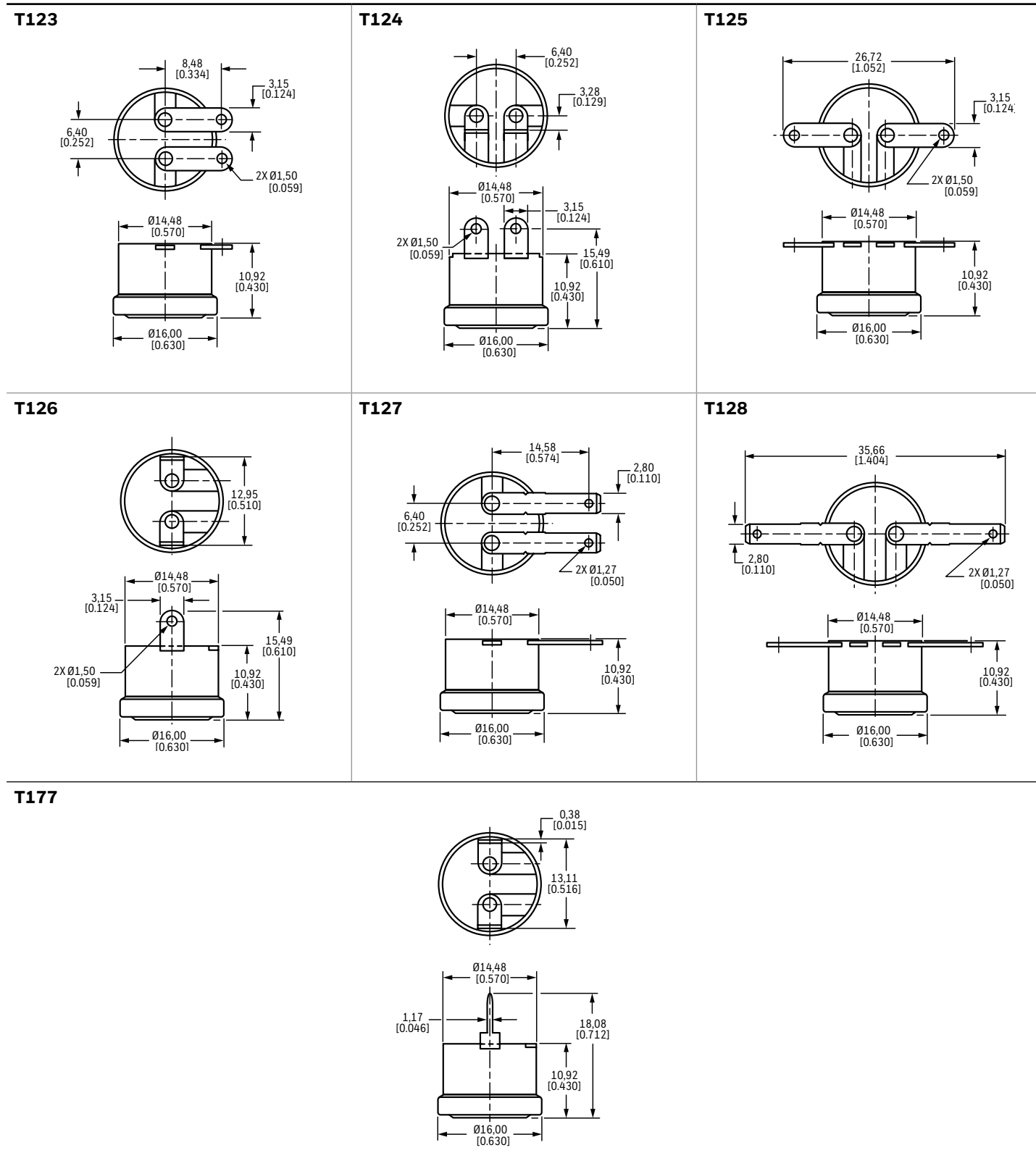
Figure 8: 3004 Series Terminals
