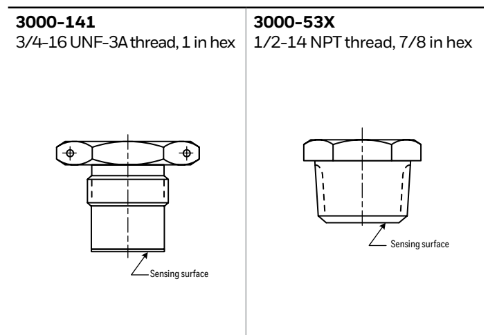
Figure 13: 3000 Series Housings: Used with Terminations 1, 2a, 2b only
