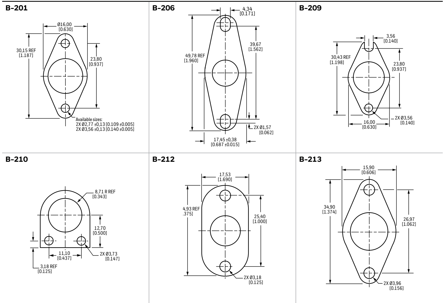
Figure 4: 3001/3004 Series Brackets
