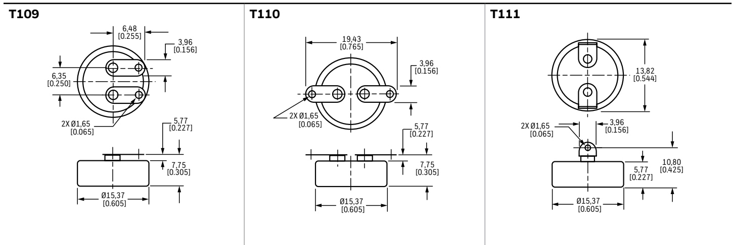
Figure 10: 3150/3156 Series Terminals
