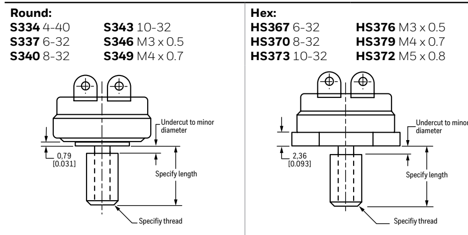
Figure 5: 3001/3004 Series Cap Studs
