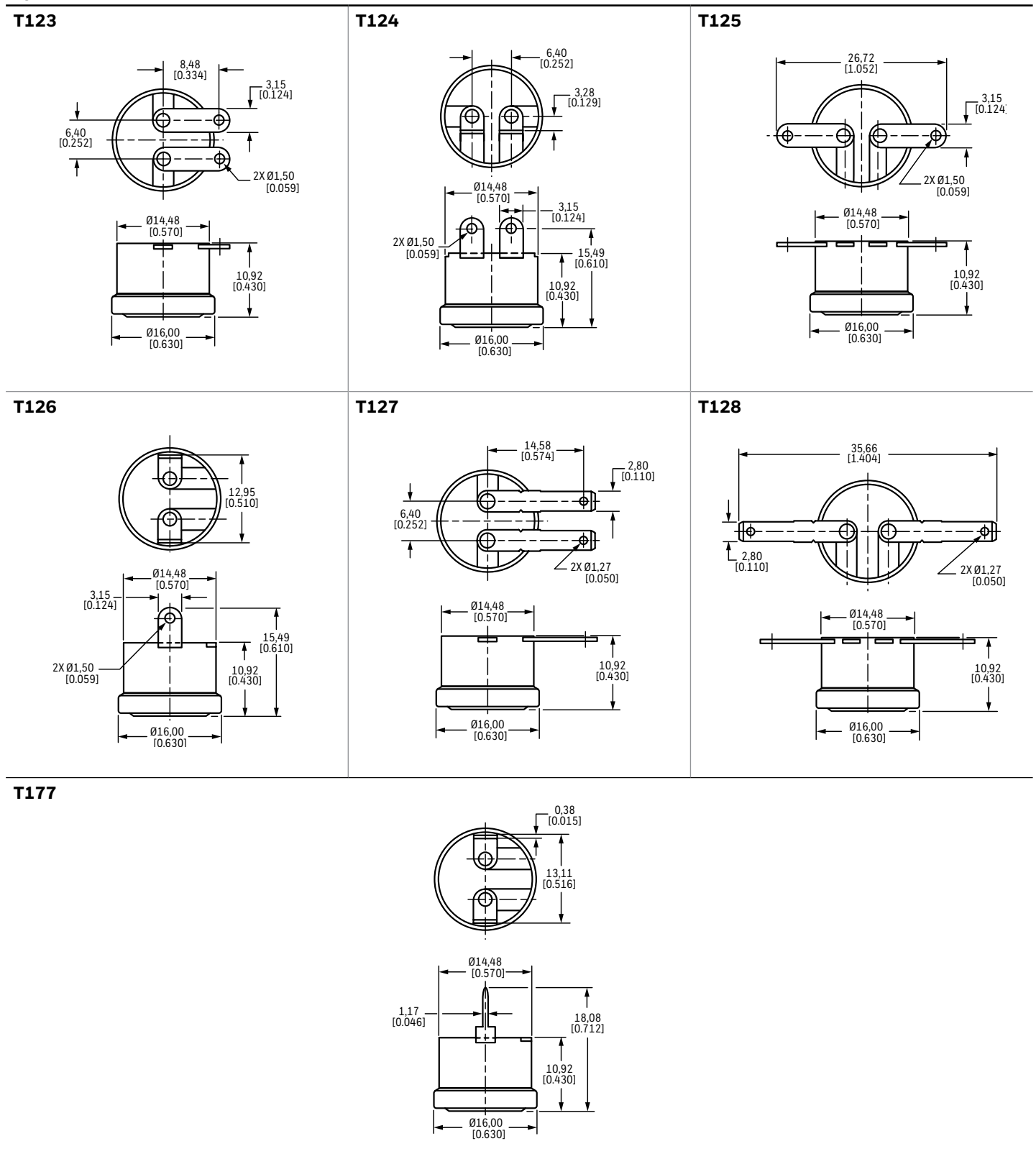
Figure 8: 3004 Series Terminals
