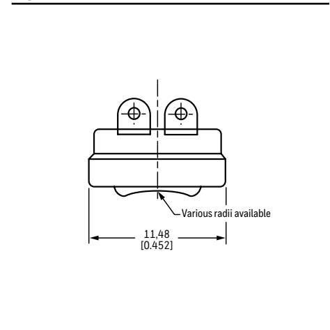
Figure 6: 3001/3004 Series Radius Cap
