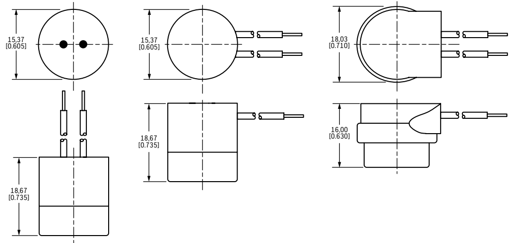
Figure 14: Overmolds Used on All Series (3100/3106 Shown)
