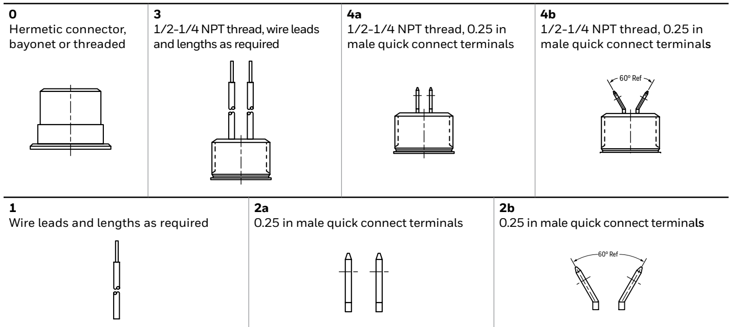
Figure 11: 3000 Series Terminations
