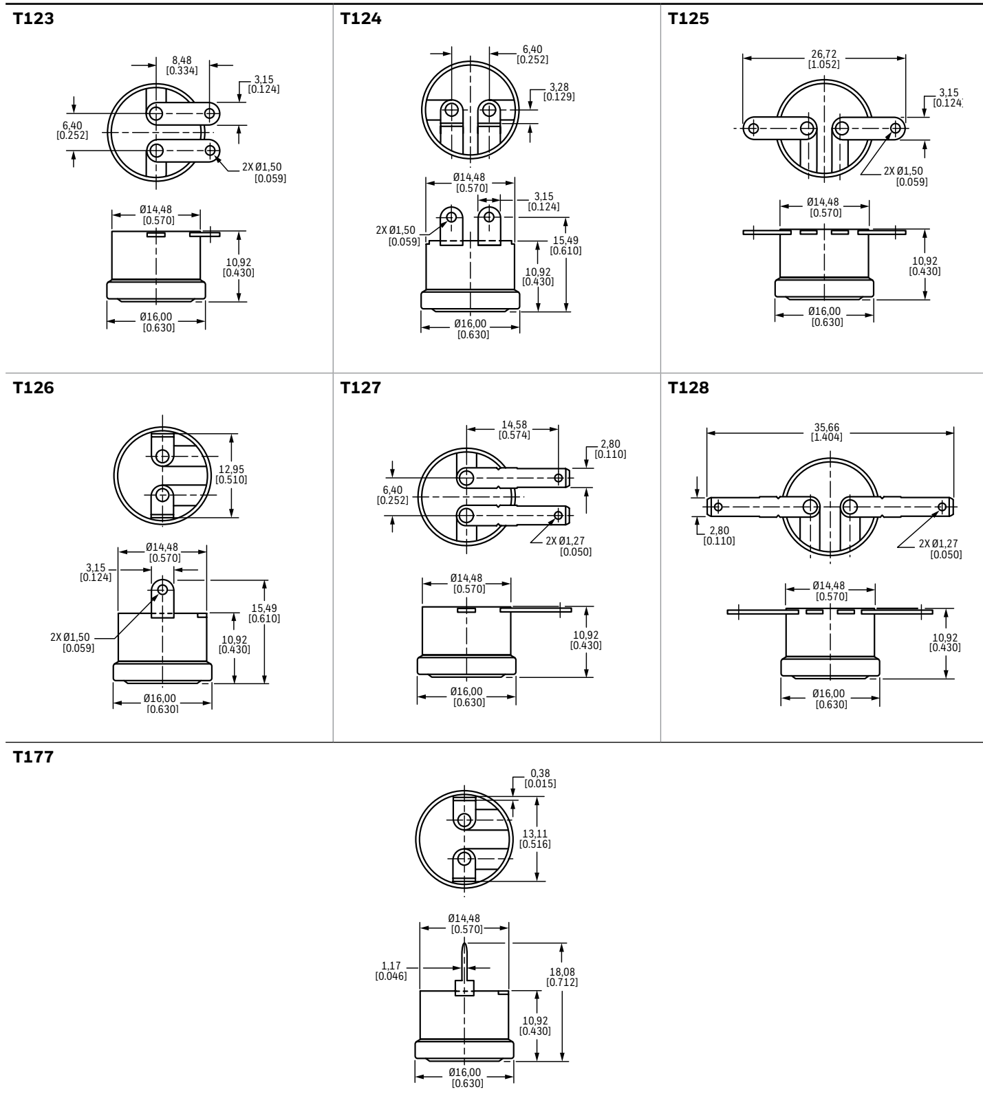
Figure 8: 3004 Series Terminals
