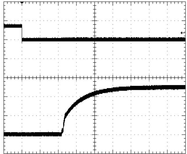
Fig-5: Turn-on transient at full rated load current (resistive) plus 20,000µF at Vin=48V, triggered via ON/OFF pin. Top trace: ON/OFF signal (5V/div). Bottom trace: output voltage (2V/div). Time scale: 10ms/div
