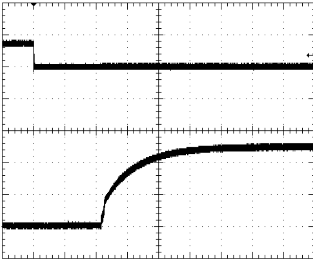
Fig-4: Turn-on transient at full rated load current (resistive) with 10µF tantalum + 1µF ceramic capacitor at Vin=48V, triggered via ON/OFF pin. Top trace: ON/OFF signal (5V/div). Bottom trace: output voltage (2V/div). Time scale: 2ms/div
