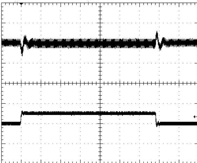
Fig-6: Output voltage response to load current step-change (20A-30A-20A) at Vin=48V. Top trace: Output voltage (200mV/div). Bottom trace: load current (20A/div). Current slew rate: 5A/µs. Co=470µF Low Z EL-con + 10µF ceramic. Time scale: 200µs/div
